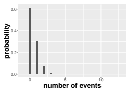
(a) \lambda = 0.5
