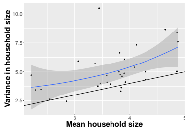
(b) Loess smoother
