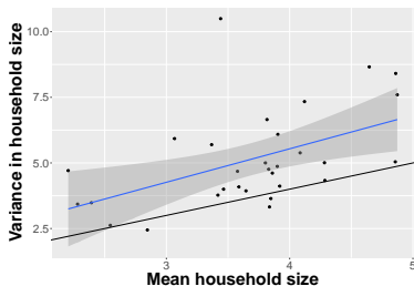
(a) Linear fit
