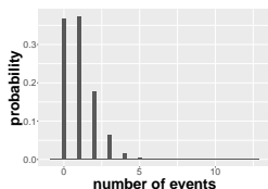
(b) \lambda = 1
