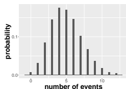
(c) \lambda = 5
