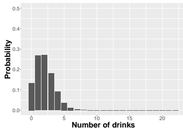
(b) Poisson distribution with same mean
