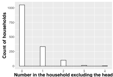
(a) Distribution of number of children under 5 in households across all 5 Philippine regions.
