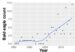
(b) Bald eagle counts vs. year
